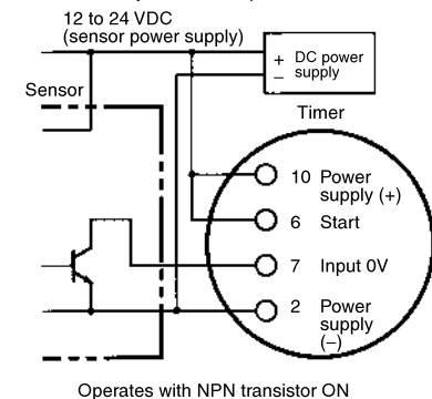
Operates with NPN transistor ON
