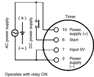
Operates with relay ON
