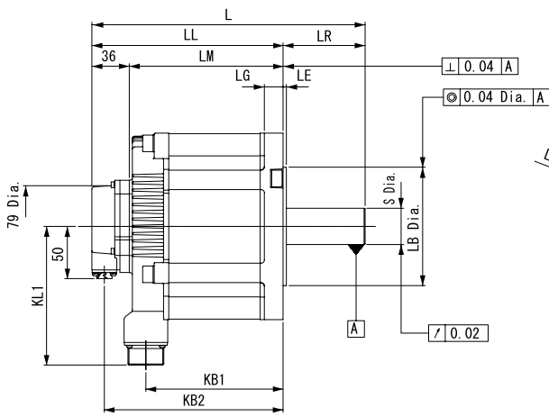
Models without brake
