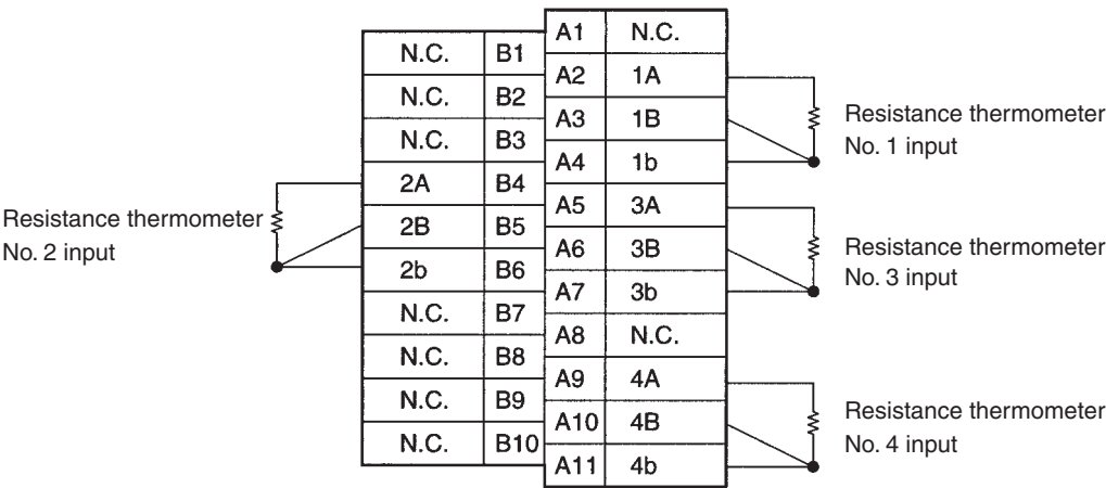
CS1W-PTS02 Isolated-type Resistance Thermometer Unit
