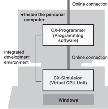
System PLC CS1
