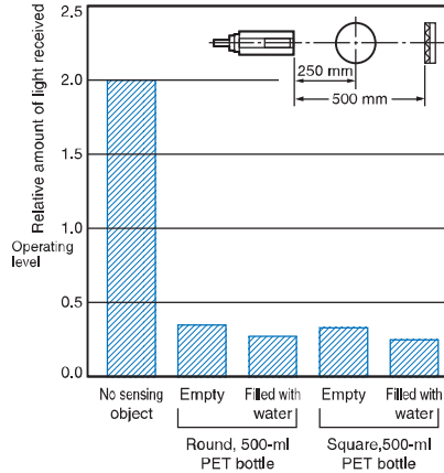
Transparent detected with P-opaqing function E3F□-B□1
